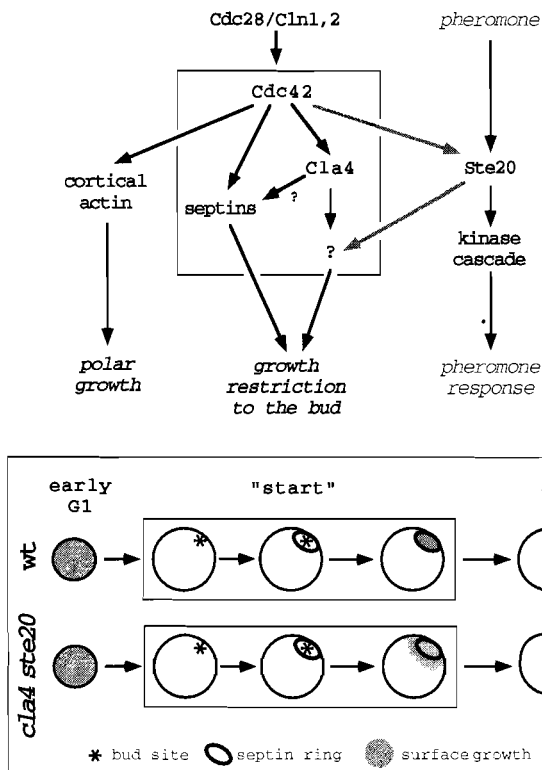
Figure 8. Cla4 and Ste20 share a role in establishing the border between mother cell and its bud, an event controlled by Cln1 and Cln2. The interaction between Cla4 and Cdc42 may be required for colocalization of active Cla4 kinase and the septin ring—two components contributing to the restriction of cell growth to the bud.
