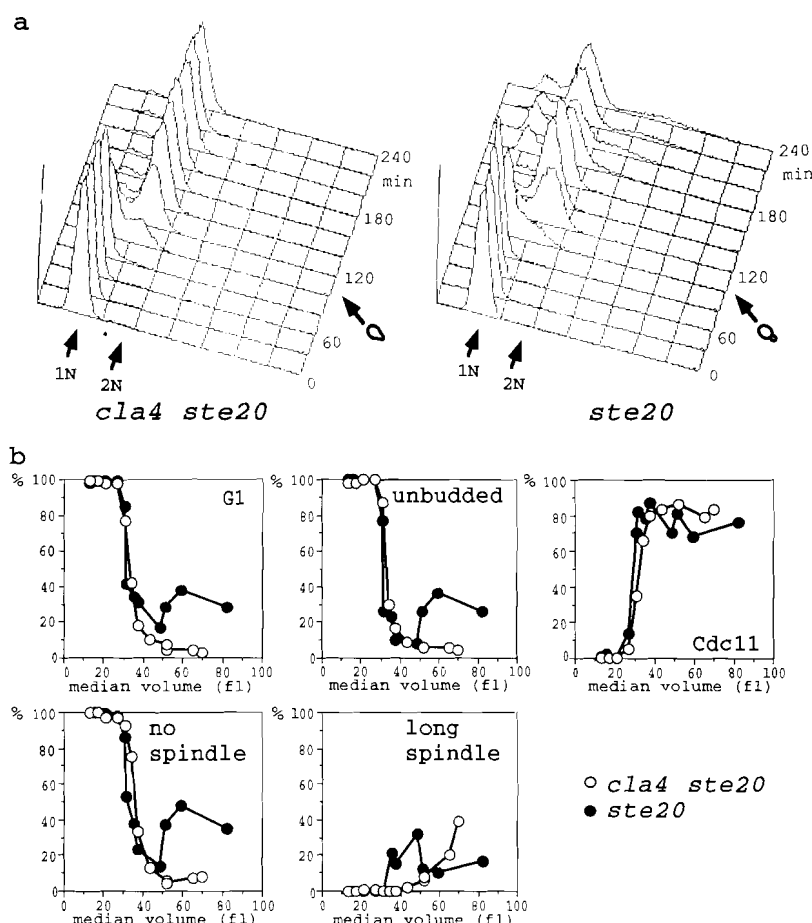
Figure 5. cla4-75 ste20 cells (K4580) and CLA4 ste20 cells (K3621) were synchronized by centrifugal elutriation and released at 37°C (the restrictive temperature for cla4-75 ). DNA replication was followed by FACS analysis; fractions of unbudded cells, cells with mitotic spindles of various stages, and Cdc11-containing structures were determined microscopically. (a) cla4-75 ste20 and CLA4 ste20 cells undergo DNA replication and acquire polarized shape at the same time (arrows denote the time when half of the culture budded). (b) Initiation of DNA replication, local accumulation of Cdc11, budding, and mitotic spindle formation occur at a comparable cell size in mutant and control cells, whereas spindle elongation is delayed in the cla4-75 ste20 mutant.
